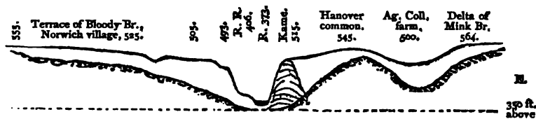
FIG. 87.—Section across the Connecticut Valley, from Norwich, Vermont, to Hanover, New Hampshire, distance three miles. The kame is nearly covered by later river silt. (Upham.)
